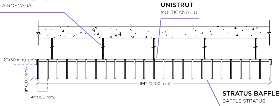
CABLE TO UNISTRUT VARILLA ROSCADA
