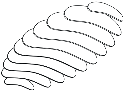
snow grains
