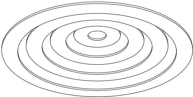
freezing
