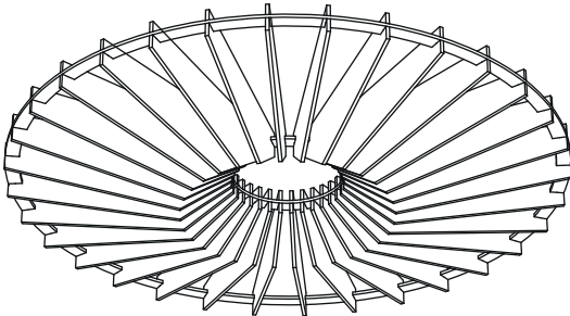
drizzle
